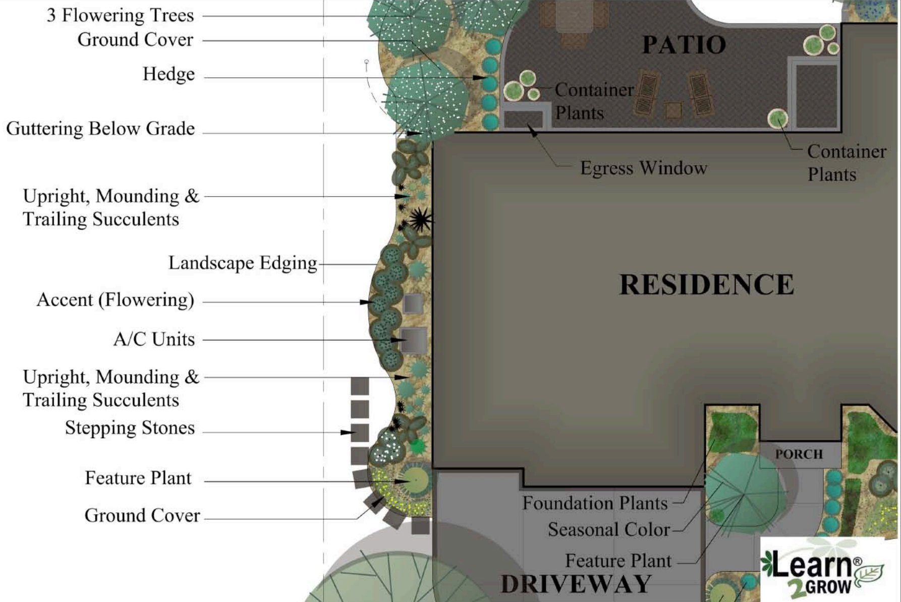
LANDSCAPE ARCHITECTURAL SITE PLAN SUCCULENT GARDEN
