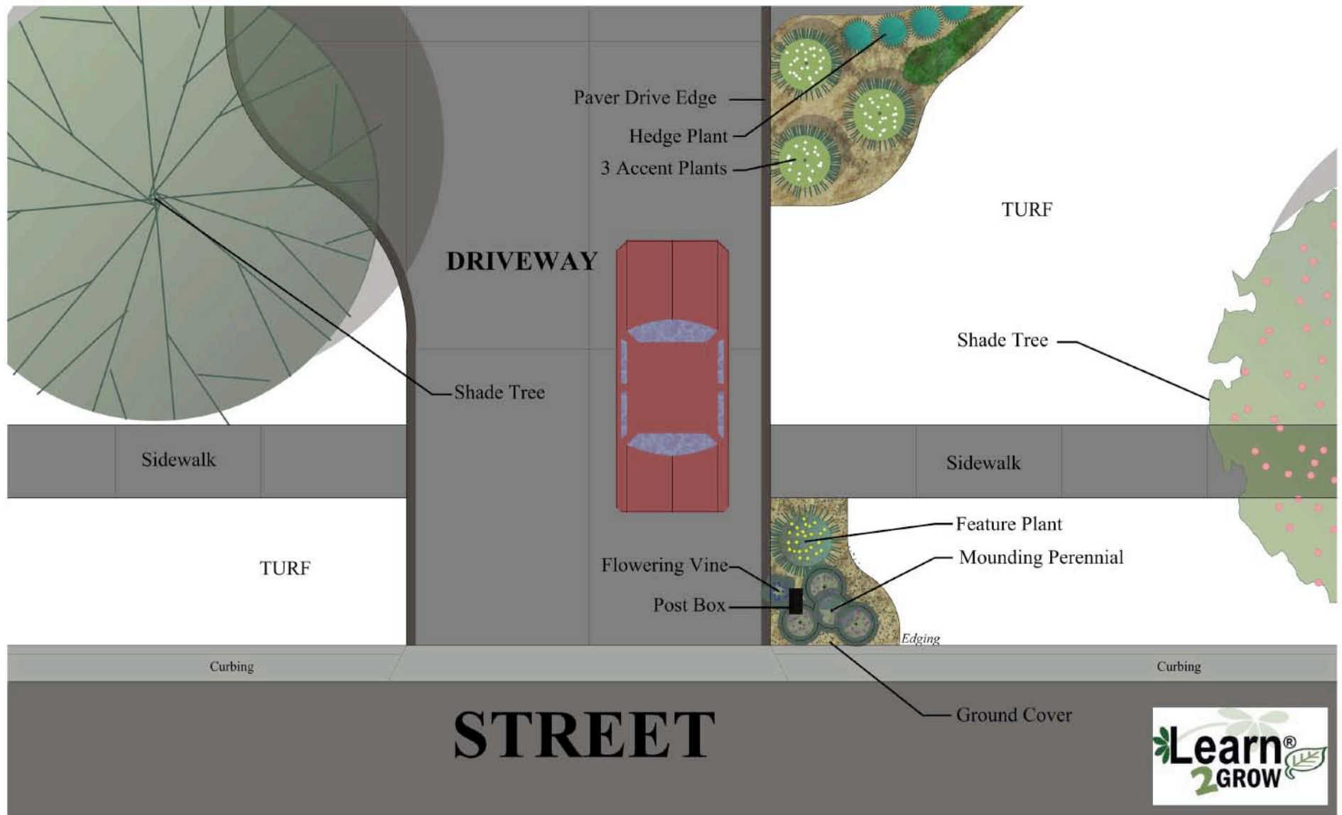
LANDSCAPE ARCHITECTURAL SITE PLAN MAILBOX PLANTING
